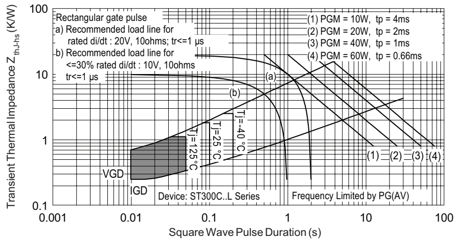
Fig. 10 - Thermal Impedance Z_{th-hs} Characteristics
