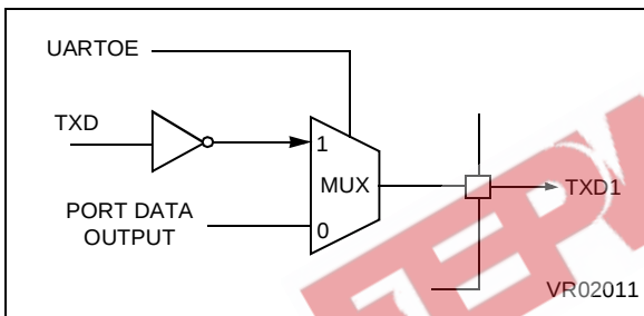
Figure 37. UART Data Output
