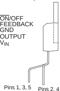
KV (TO-220 STAGGERED LEADS) PACKAGE (TOP VIEW)
