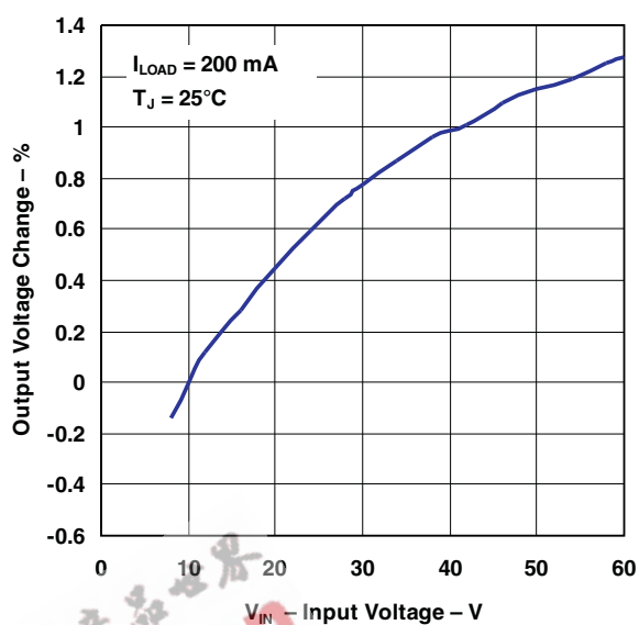
Figure 4. Line Regulation
