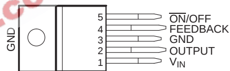
KV (TO-220 STAGGERED LEADS) PACKAGE (TOP VIEW)
