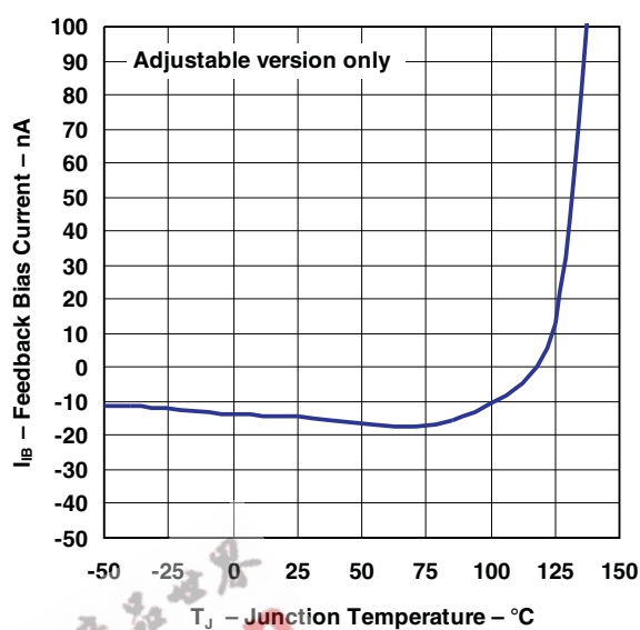
Figure 12. FEEDBACK Current
