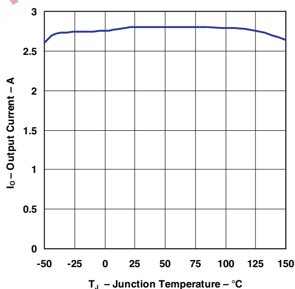
Figure 6. Current Limit
