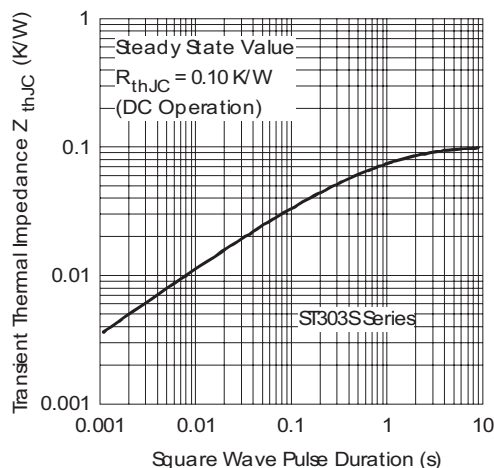
Fig. 8 - Thermal Impedance Z_{\theta JC} Characteristics
