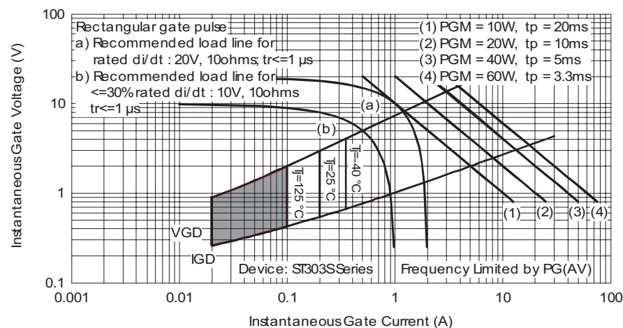
Fig. 15 - Gate Characteristics
