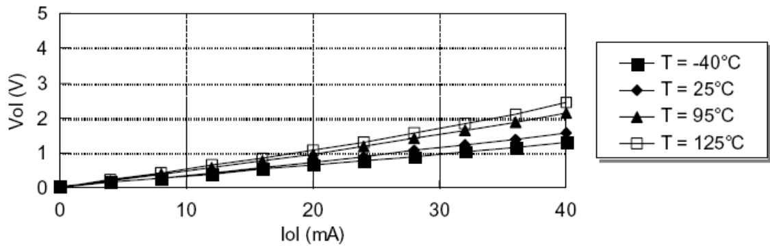
Figure 34. Vol versus Iol for High sink (30mA) I/O ports at Vdd=5V
