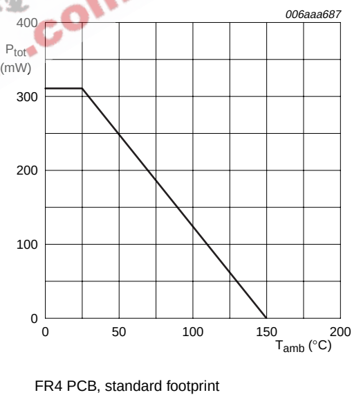
Fig 4. Power derating curve
