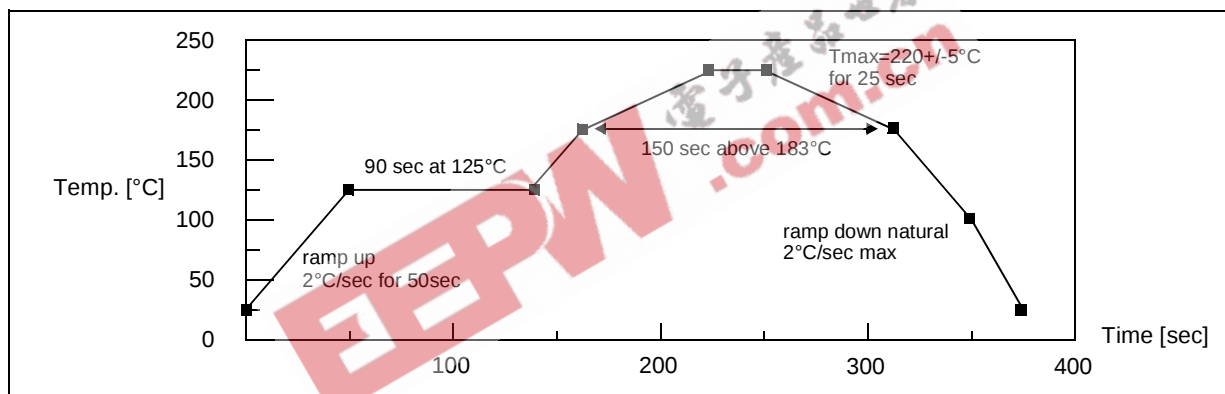
Figure 73. Recommended Reflow Soldering Oven Profile (MID JEDEC)
