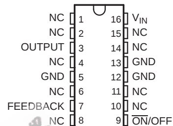
N (PDIP) PACKAGE (TOP VIEW)
