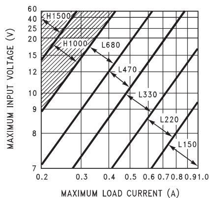
Figure 16. TL2575-50
