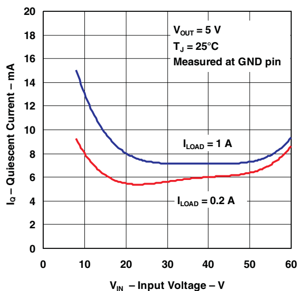
Figure 7. Quiescent Current
