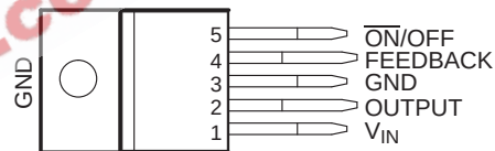
KV (TO-220 STAGGERED LEADS) PACKAGE (TOP VIEW)
