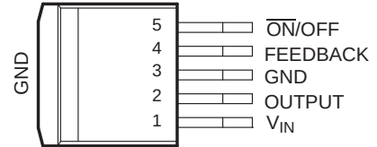
KT (TO-263) PACKAGE (TOP VIEW)
