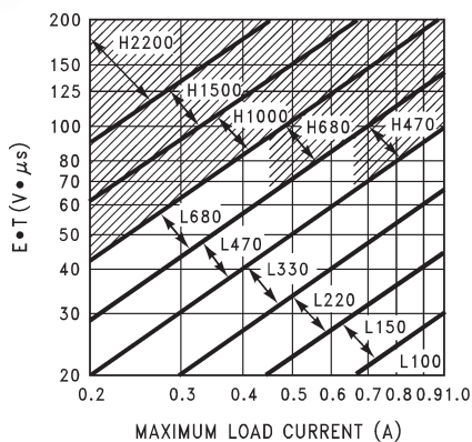
Figure 19. TL2575-ADJ
