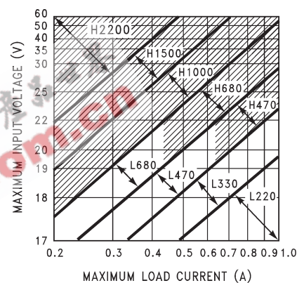
Figure 18. TL2575-15
