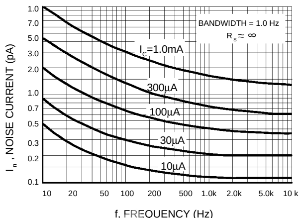
Figure 2. Noise Current
