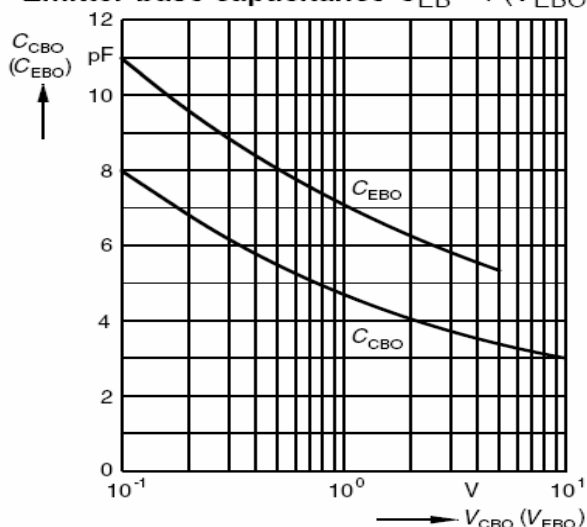
Collector-base capacitance C_{CB} = f(V_{CBO}) Emitter-base capacitance C_{EB} = f(V_{EBO})
