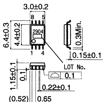
BA2904FV(SS0P-B8) (Unit:[mm])
