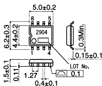
BA2904F(S0P8) (Unit:[mm])
