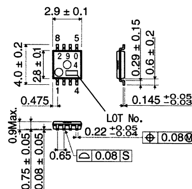
BA2904FVM(MSOP8) (Unit : [mm])
