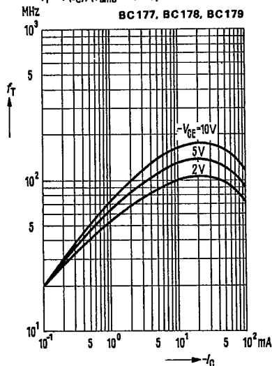
Transition frequency f_T = f(f_C); (T_{amb} = 25^\circ\text{C})
