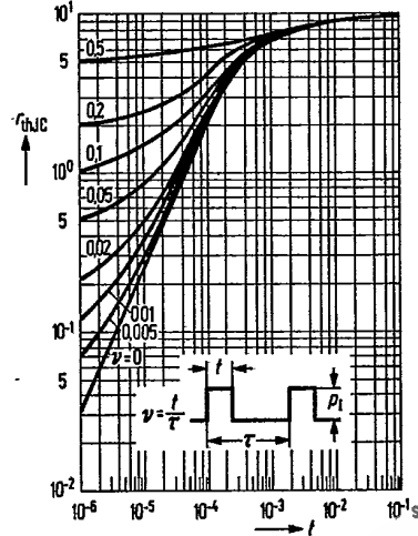
Permissible pulse load r_{\text{thJC}} = f(t); v = \text{parameter} BD 136, BD 138, BD 140
