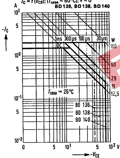
Permissible operating range I_C = f(V_{\text{CE}}); (T_{\text{case}} = 60^\circ\text{C}); v = 0 BD 136, BD 138, BD 140
