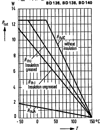
Total perm. power dissipation versus temperature P_{\text{tot}} = f(T); R_{\text{th}} = \text{parameter} BD 136, BD 138, BD 140
