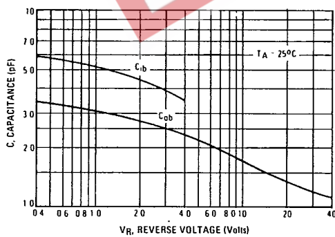
FIGURE 5 - CAPACITANCES
