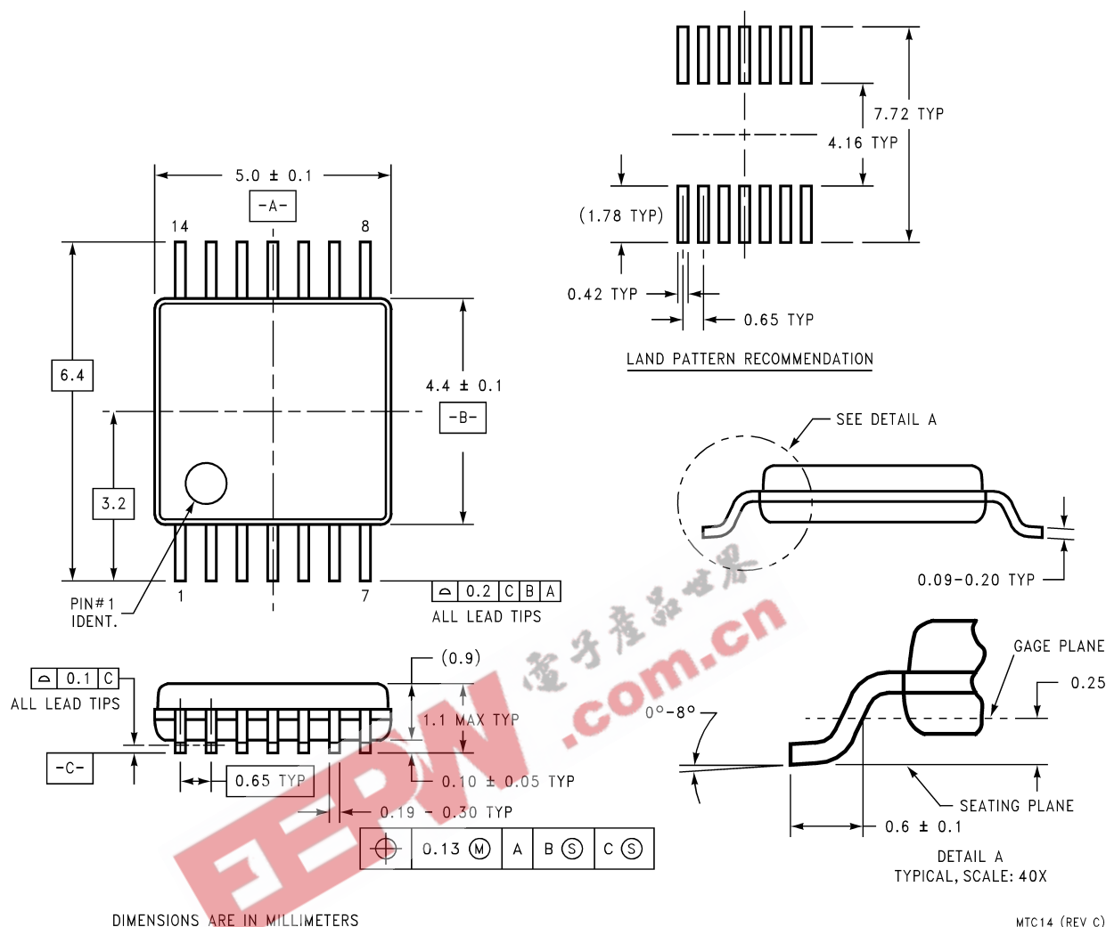
TSSOP-14 Pin Package NS Package Number MTC14
