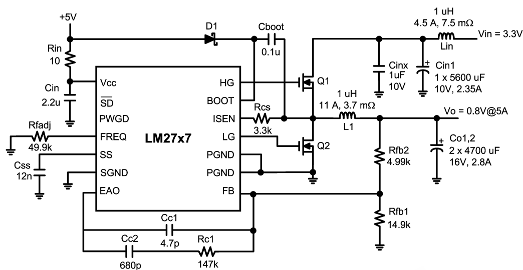
FIGURE 5. 3.3V to 0.8V, 5A, 500kHz
