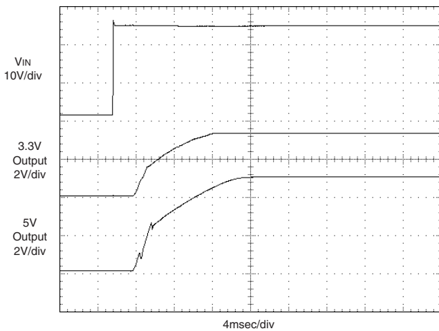
Start-Up from VIN (VIN = 24V, 5V @ 7.5A, 3.3V @ 7.5A, external 10μF || 1μF output capacitors.)
