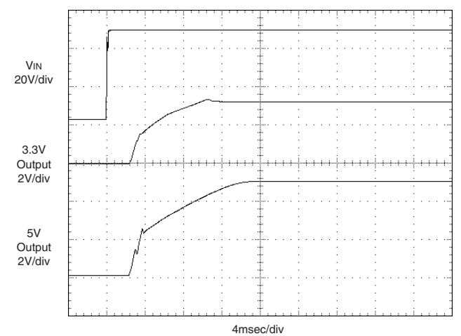
Start-Up from VIN (VIN = 48V, 5V @ 7.5A, 3.3V @ 7.5A, external 10μF || 1μF output capacitors.)
