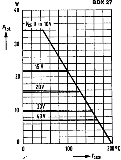
Total perm. power dissipation versus temperature P_{\text{tot}} = f(T_{\text{case}}); V_{\text{CE}} = \text{parameter}
