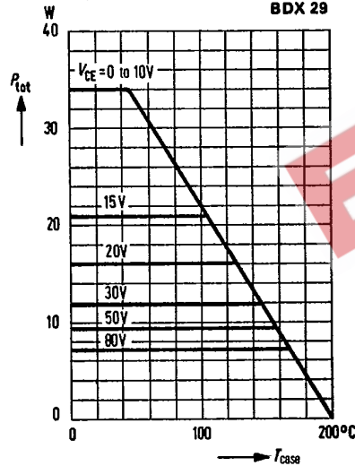
Total perm. power dissipation versus temperature P_{\text{tot}} = f(T_{\text{case}}); V_{\text{CE}} = \text{parameter}
