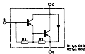
BDX54 Series PNP
