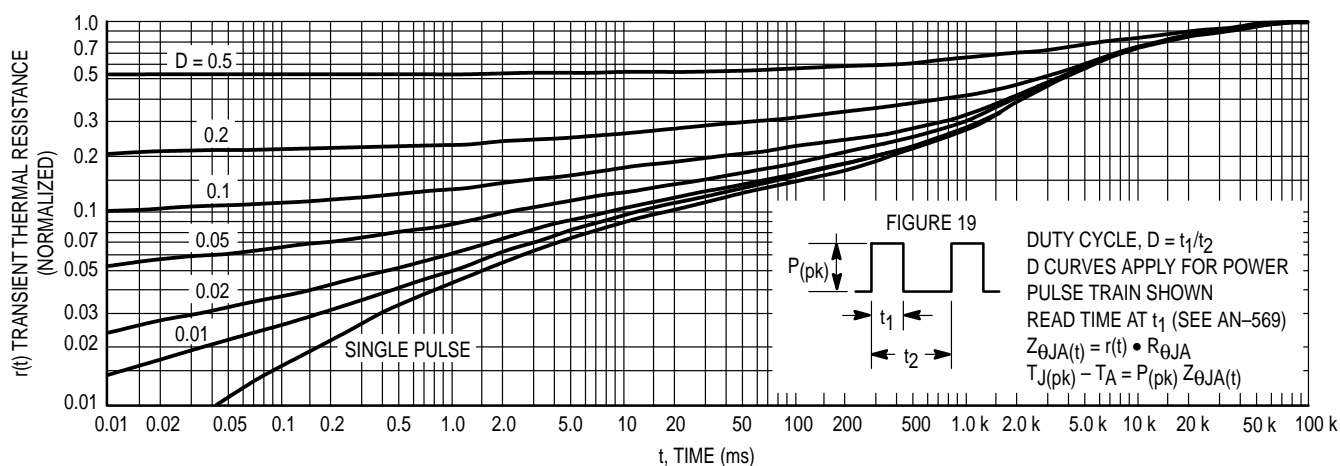
Figure 17. Thermal Response
