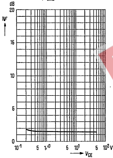
Noise figure NF = f(V_{CE}) I_G = 0.2 \text{ mA}; R_G = 2 \text{ k}\Omega; f = 1 \text{ kHz} \Delta f = 200 \text{ Hz}; T_{\text{amb}} = 25^\circ \text{C}
