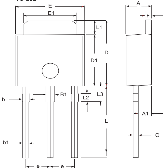
TO-251
