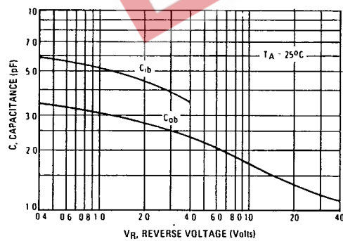
FIGURE 5 - CAPACITANCES
