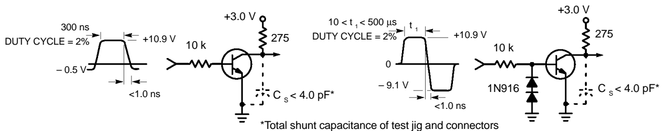
Figure 2. Turn–Off Time
