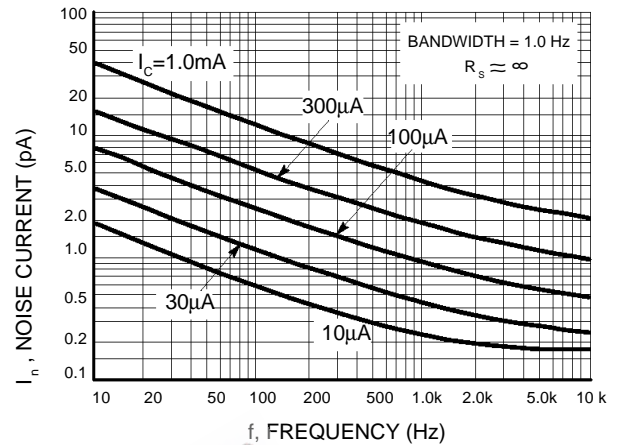
Figure 4. Noise Current
