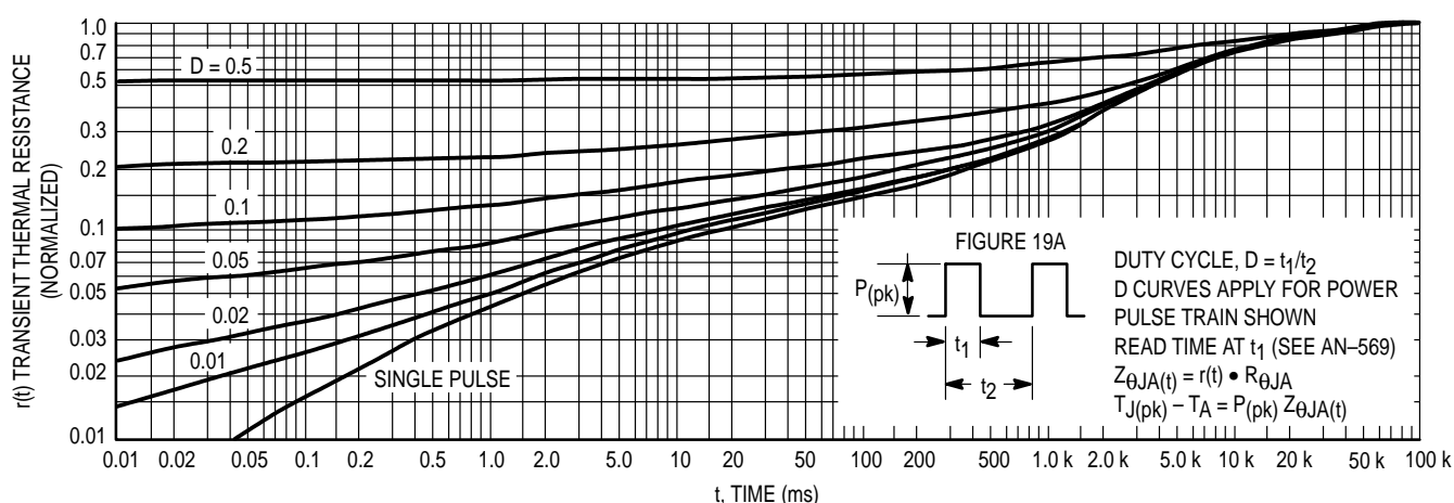
Figure 19. Thermal Response
