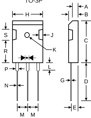
TO-3P
