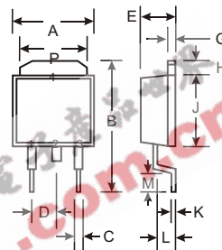
TO-252 / DPAK
