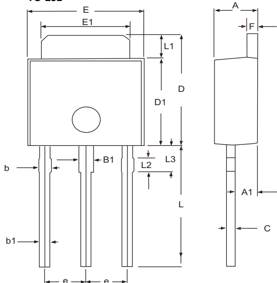
TO-251
