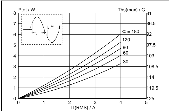
Fig.1. Maximum on-state dissipation, P tot , versus rms on-state current, I T(RMS) , where α = conduction angle.
