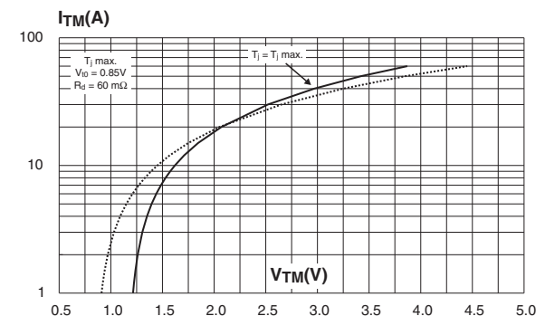
Figure 4: On-state characteristics (maximum values)
