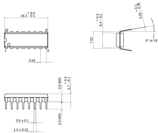
PACKAGE STRUCTURE
