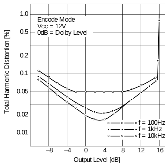
NR on Total Harmonic Distortion-1 (CXA1101)
