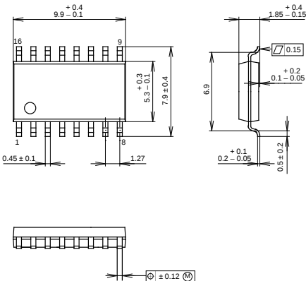
PACKAGE STRUCTURE
