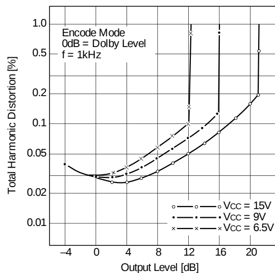
NR on Total Harmonic Distortion-4 (CXA1102)
