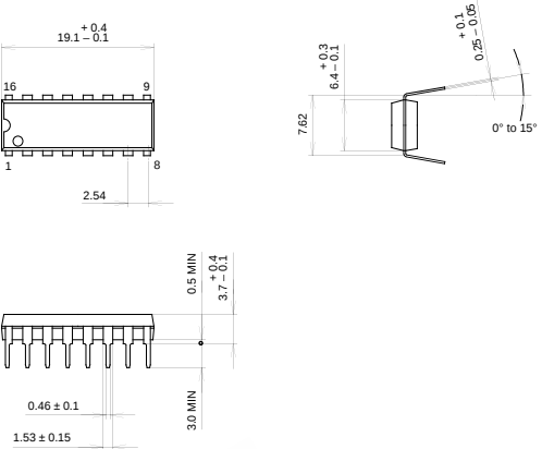
PACKAGE STRUCTURE
