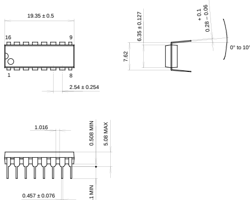
PACKAGE STRUCTURE
