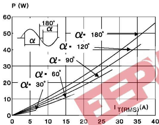
Fig.3 : Maximum RMS power dissipation versus RMS on-state current ( F=50\text{Hz} ).
