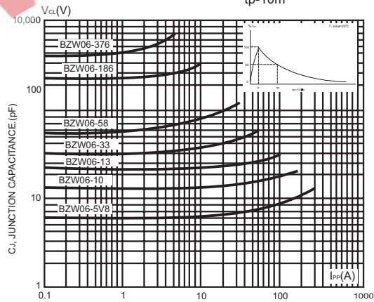
FIG.4- CLAMPING VOLTAGE VERSUS PEAK PULSE CURRENT. EXPONENTIAL WAVEFORM t_p=200\mu\text{s} , t_p=1\text{ms} , t_p=10\text{ms}
