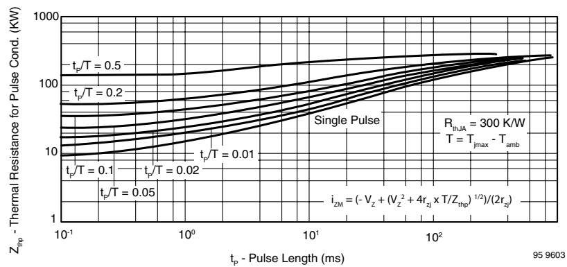
Figure 11. Thermal Response
