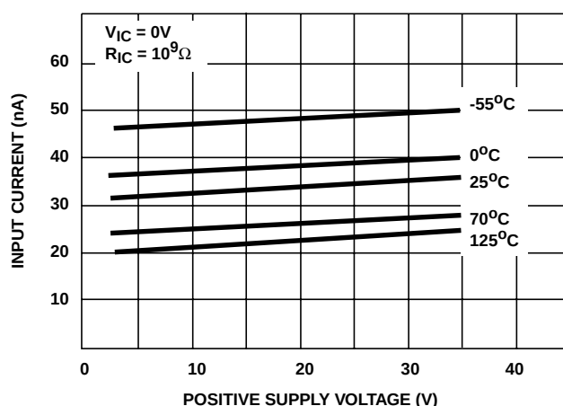
FIGURE 2. INPUT CURRENT vs SUPPLY VOLTAGE
