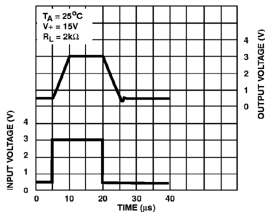
FIGURE 7. VOLTAGE FOLLOWER PULSE RESPONSE (LARGE SIGNAL)
