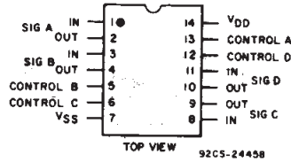
TOP VIEW 92CS-2445B
