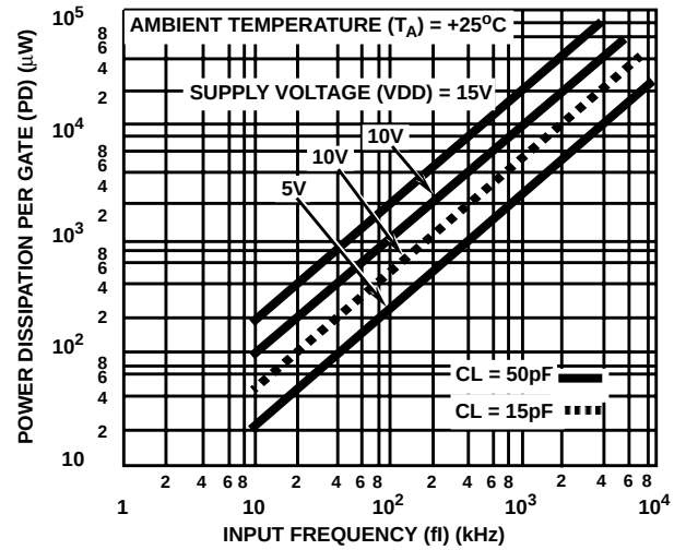
FIGURE 2. TYPICAL POWER DISSIPATION vs FREQUENCY
