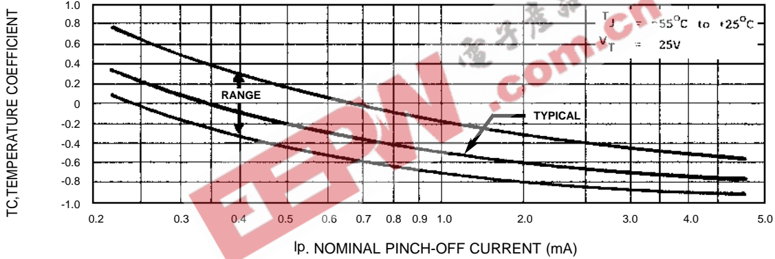
FIGURE 3 TEMPERATURE COEFFICIENT
