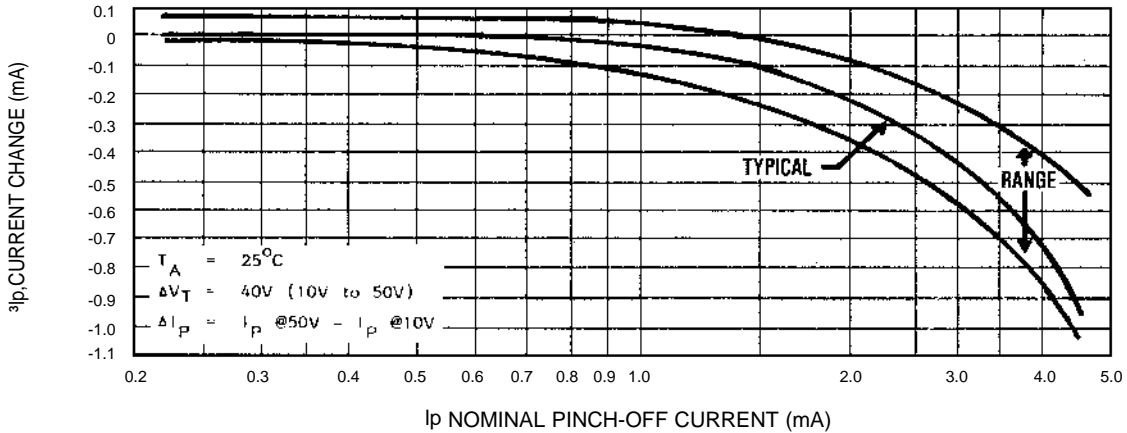
FIGURE 4 TEMPERATURE COEFFICIENT
