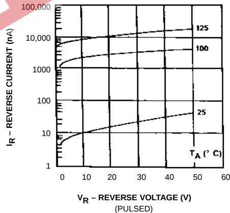
Figure 4. CD5711 Typical Variation of Reverse Current ( I_R ) vs. Reverse Voltage ( V_R ) at Various Temperatures.
