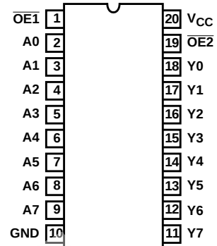
CD54HC541, CD54HCT541 (CERDIP) CD74HC541 (PDIP, SOIC, TSSOP) CD74HCT541 (PDIP, SOIC) TOP VIEW
