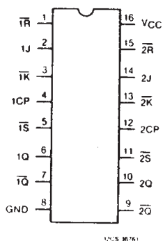
CD54/74AC/ACT109
