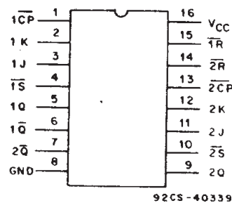
CD54/74AC/ACT112
