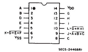
NC=NO CONNECTION
