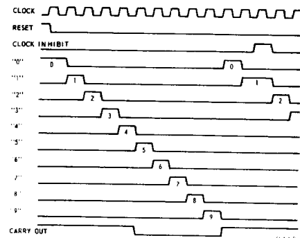
Fig. 2 - Timing diagram.
