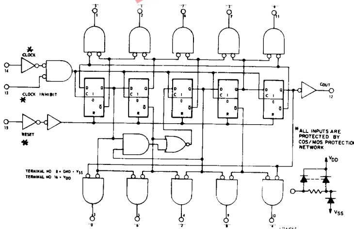
Fig. 1 - Logic diagram.
