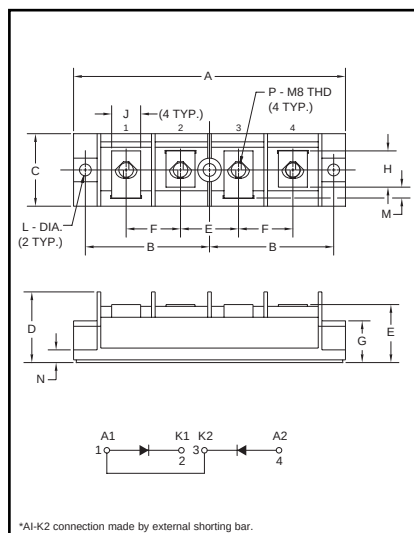
Outline Drawing
