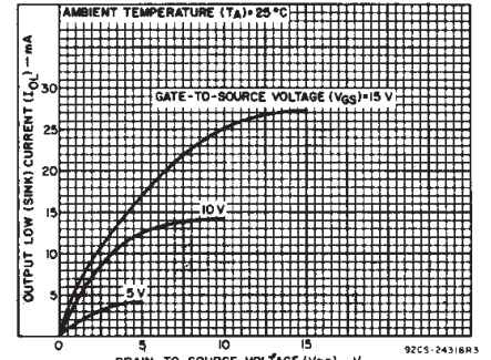
Fig. 5 - Typical output low (sink) current characteristics.
