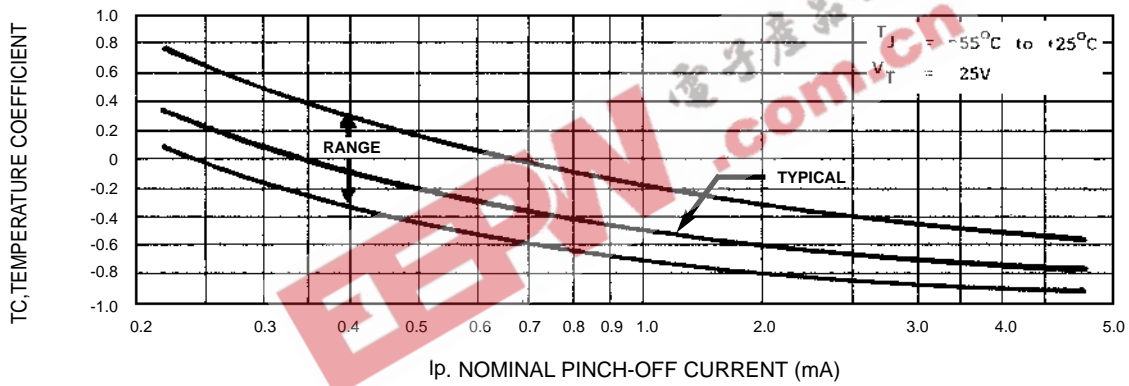
FIGURE 3 TEMPERATURE COEFFICIENT
