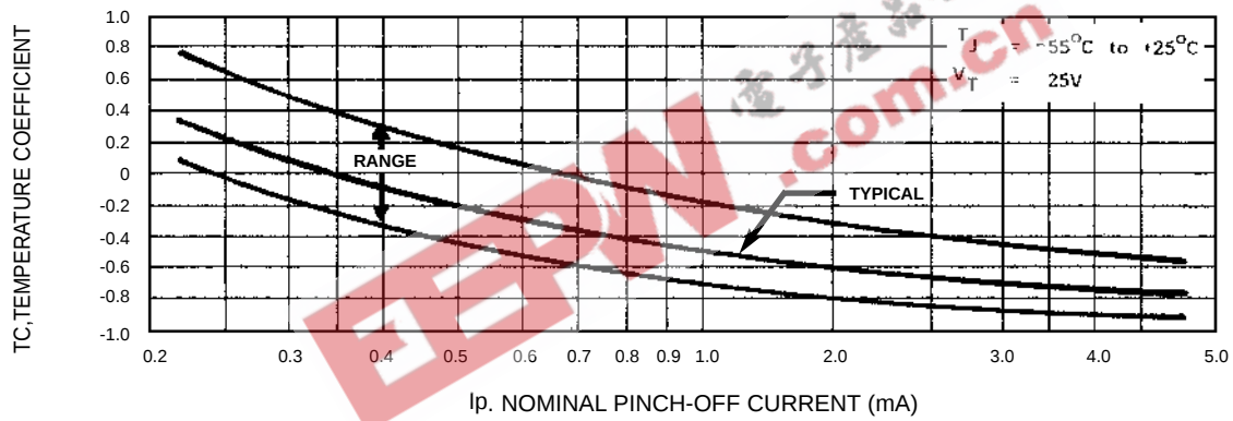
FIGURE 3 TEMPERATURE COEFFICIENT
