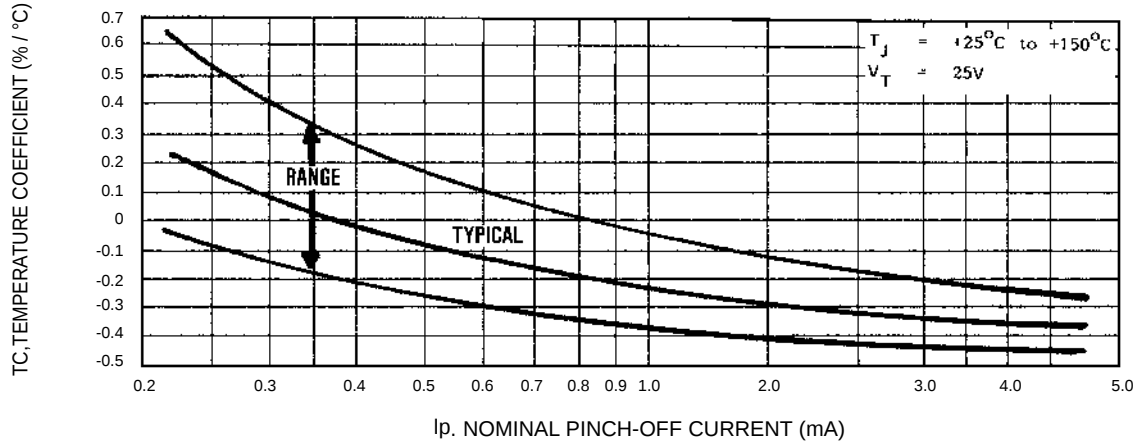
FIGURE 2 TEMPERATURE COEFFICIENT
