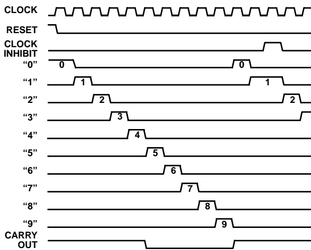
FIGURE 3. CD4017BMS
