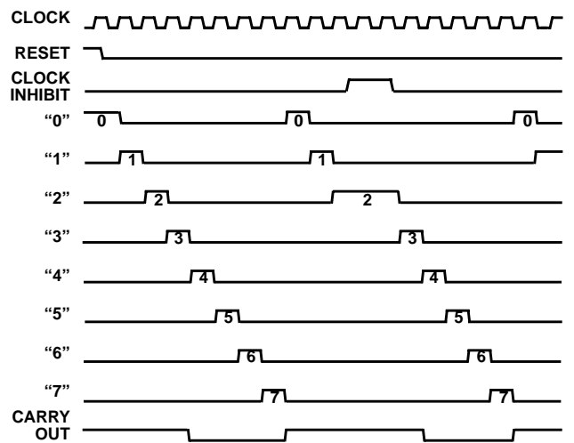
FIGURE 4. CD4022BMS
