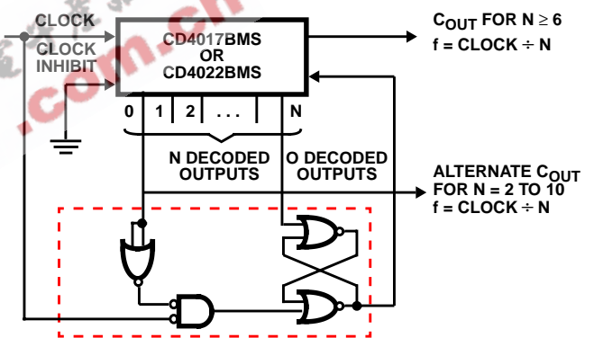
FIGURE 14. DIVIDE BY N COUNTER (N ≤ 10) WITH N DECODED OUTPUTS
