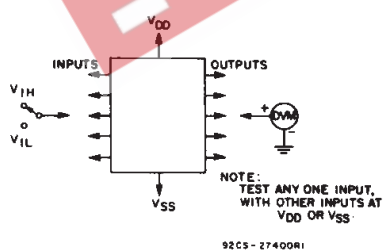
Fig. 21 - Noise immunity test circuit.
