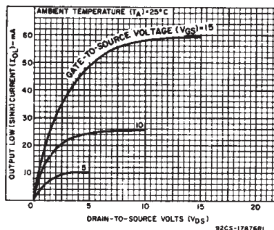
Fig. 10 - Minimum output low (sink) current characteristics.
