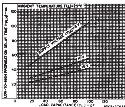
Fig. 13 - Typical low-to-high propagation time vs. load capacitance (CD4009UB).
