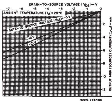
Fig. 12 - Minimum output high (source) current characteristics.
